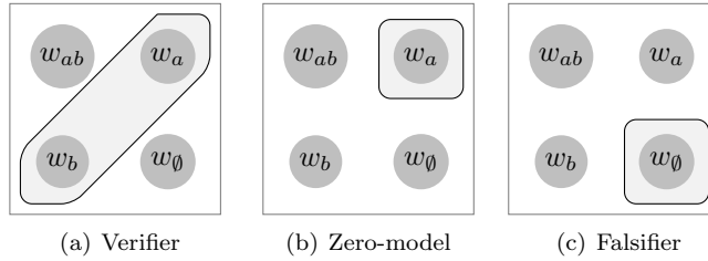
Figure 1: Models for (a \vee b) .
