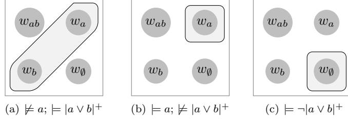
Figure 3: Illustrations of supporting states in BiUS
